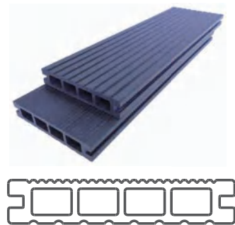
135H25-B 135*25 mm
